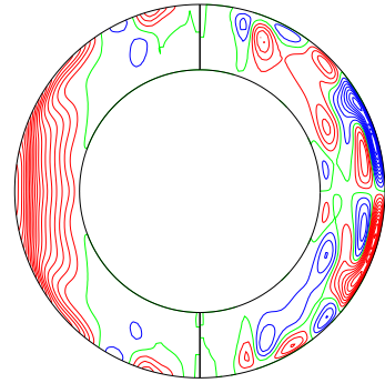
\bar{u}_\phi & merid circulation (mer) (time-average 14.88815 to 14.93815)
