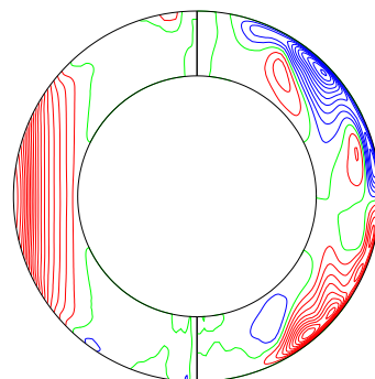
\bar{u}_\phi & merid circulation (mer) (time-average 15.23815 to 15.28815)
