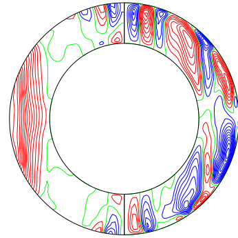
\bar{u}_\phi & merid circulation (mer) (time-average 22.37315 to 0)
