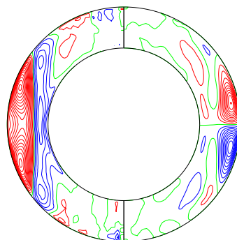
\bar{u}_\phi & merid circulation (mer) (time-average 14.80315 to 14.83815)
