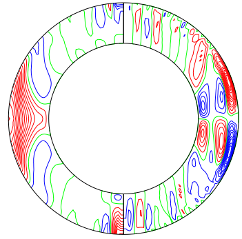
\bar{u}_\phi & merid circulation (mer) (time-average 4.200042 to 4.400044)
