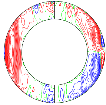
\bar{u}_\phi & merid circulation (mer) (time-average 0.3901088 to 0.4401098)
