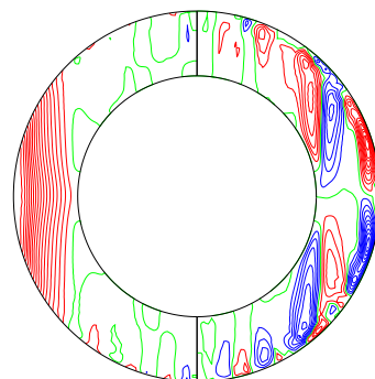
\bar{u}_\varphi & merid circulation (mer) (time-average 0.3901088 to 0.4401098)
