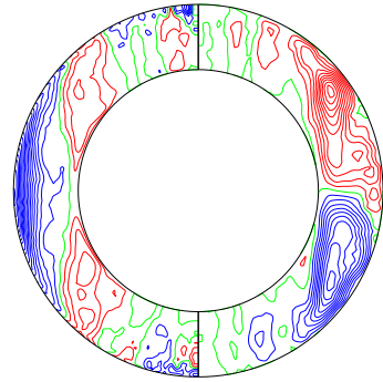
\bar{u}_\phi & merid circulation (mer) (time-average 0.6801146 to 0.6901148)
