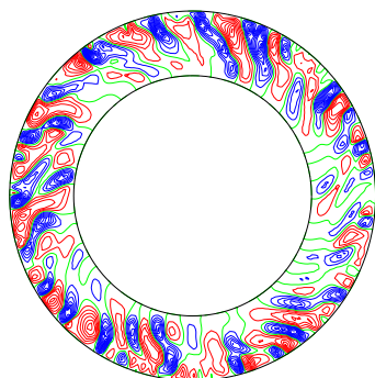
u_r (equat, last snapshot)
