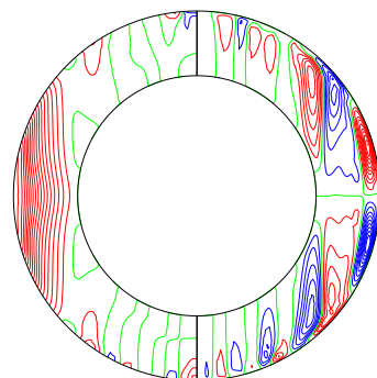
\bar{u}_\phi & merid circulation (mer) (time-average 3.140164 to 3.290167)
