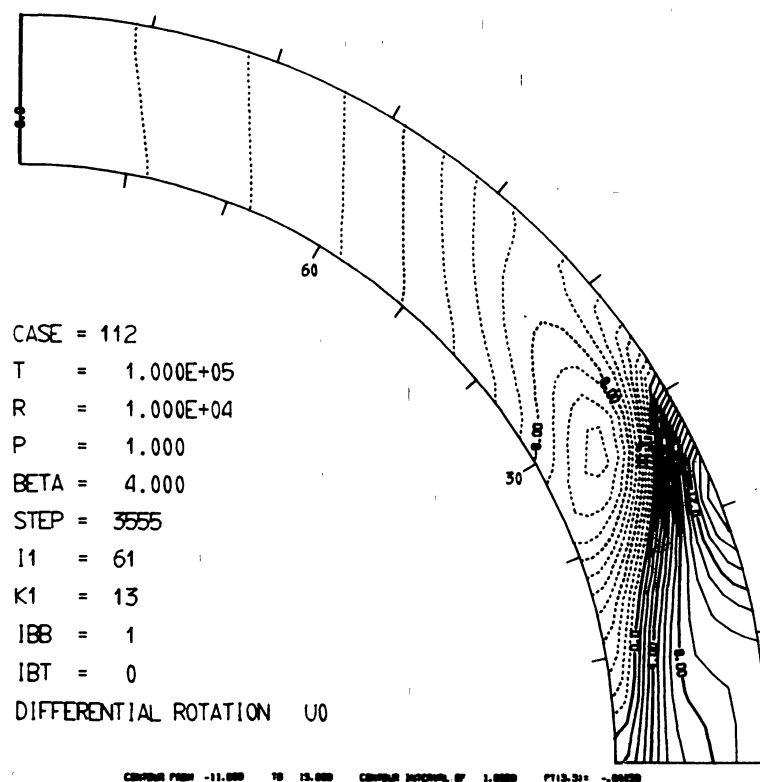
Fig. 9. Typical differential rotation profile for Rayleigh number R increased to 10^4 .
