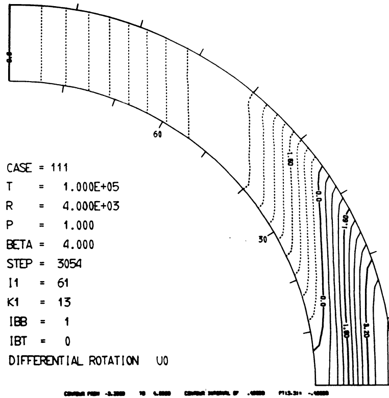
Fig. 7. Computer produced meridional cross section of linear rotation velocity u_0 relative to uniformly rotating frame, for Taylor number T = 10^5 , Rayleigh number R = 4 \times 10^3 , Prandtl number P = 1 . Units dimensionless, with velocity scaled by \kappa/d , in which \kappa is thermal diffusivity, d is convection zone depth. Positive u_0 indicated by solid contours; negative u_0 by dashed contours.
