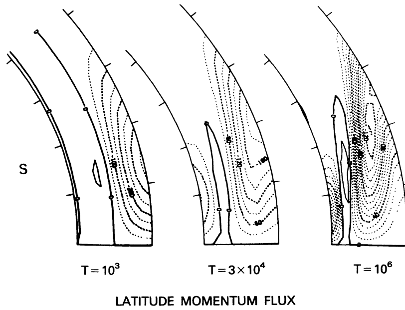
Fig. 2. Latitude-radius sections showing latitudinal angular momentum flux associated with most unstable mode m as function of Taylor number T . Dashed contours denote negative, or equatorward, momentum flux. Equatorial plane is at lower edge of each figure.
