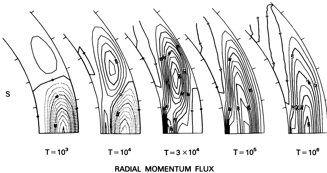
Fig. 3. Latitude-radius sections showing radial angular momentum flux associated with most unstable nodes as function of Taylor number T . Solid contours denote positive or outward momentum flux; dashed contours negative or inward flux.
