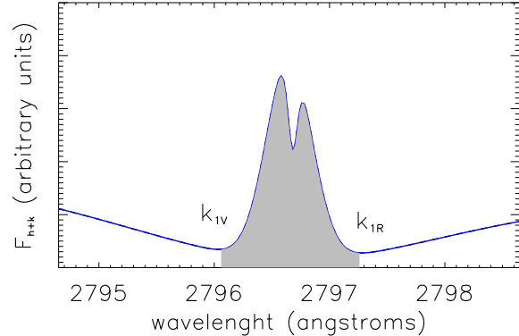
Fig. 1.— Synthetic profile of Mg II k line. The flux integration is made through the k1v and k1r minima limits.
