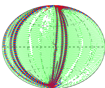
B_r at r = 0.98
