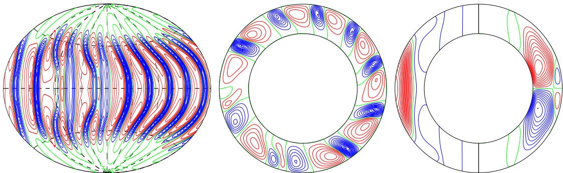
u_r at r = 0.9 u_r (equat) \bar{u}_\varphi & merid circulation (mer)
