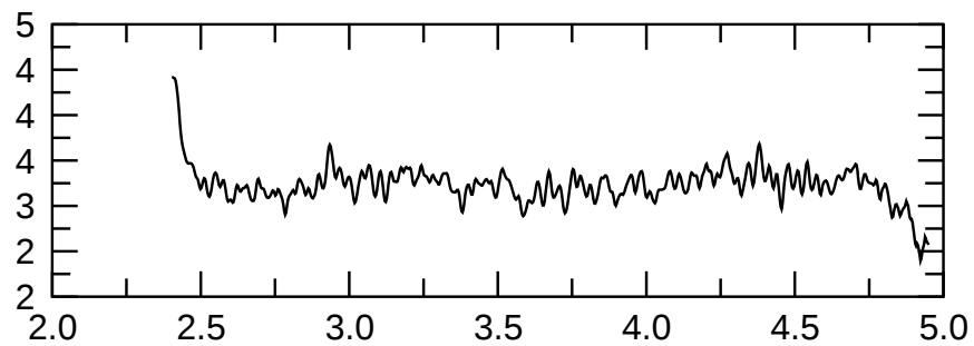
Btor( l=2, m=2 ) magn.
