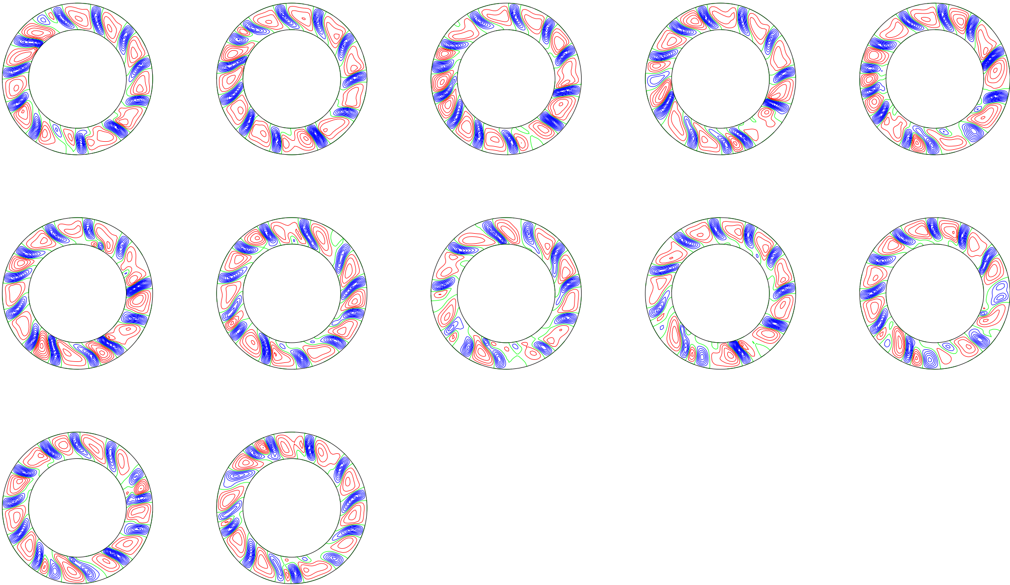
poloidal streamlines, (t[i] dt[i] t[i+1]): 3.225072 ( 0.075 ) 4.050105
