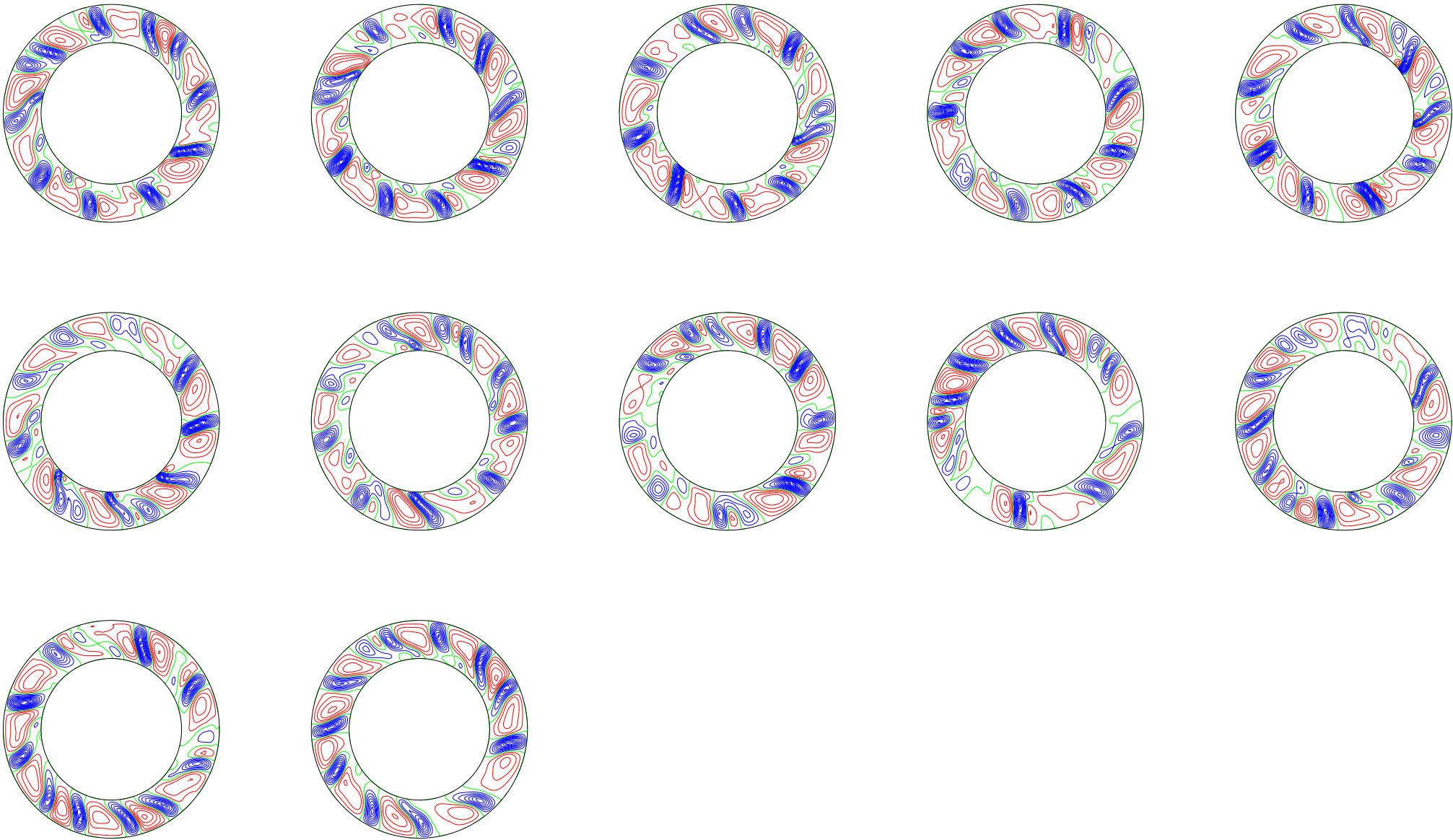
poloidal streamlines, (t[i] dt[i] t[i+1]): 4.125108 ( 0.075 ) 4.950141
