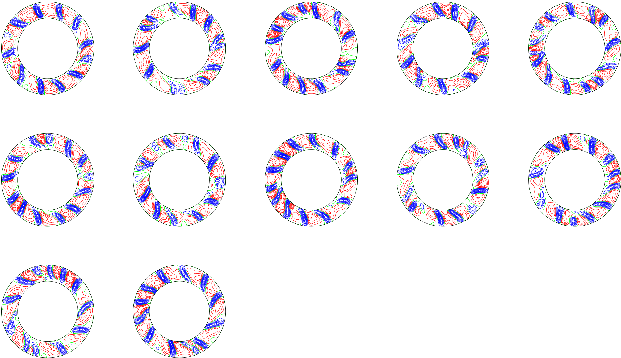
poloidal streamlines, (t[i] dt[i] t[i+1]): 2.625057 ( 0.075 ) 3.45009
