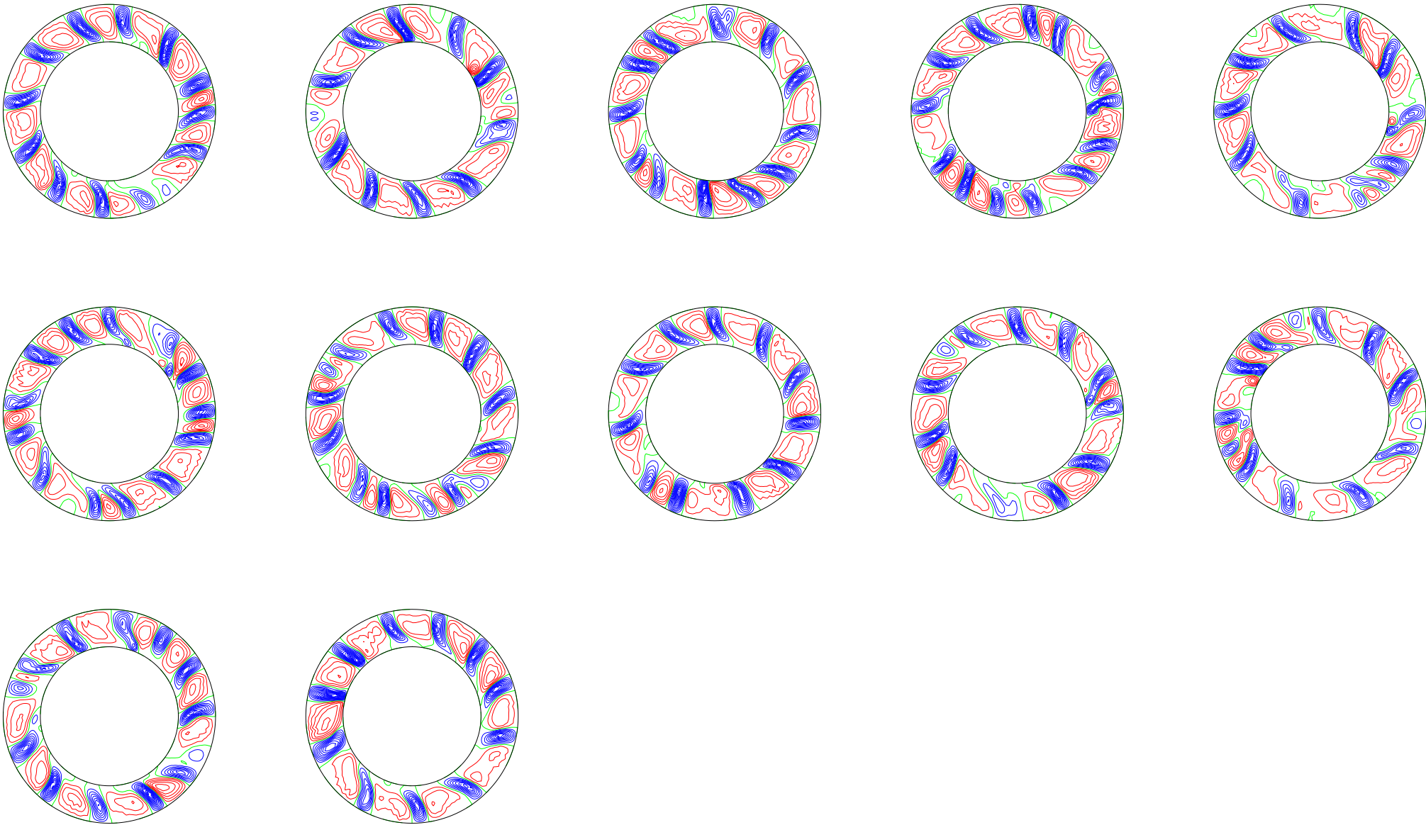
poloidal streamlines, (t[i] dt[i] t[i+1]): 2.70006 ( 0.1 ) 3.800104
