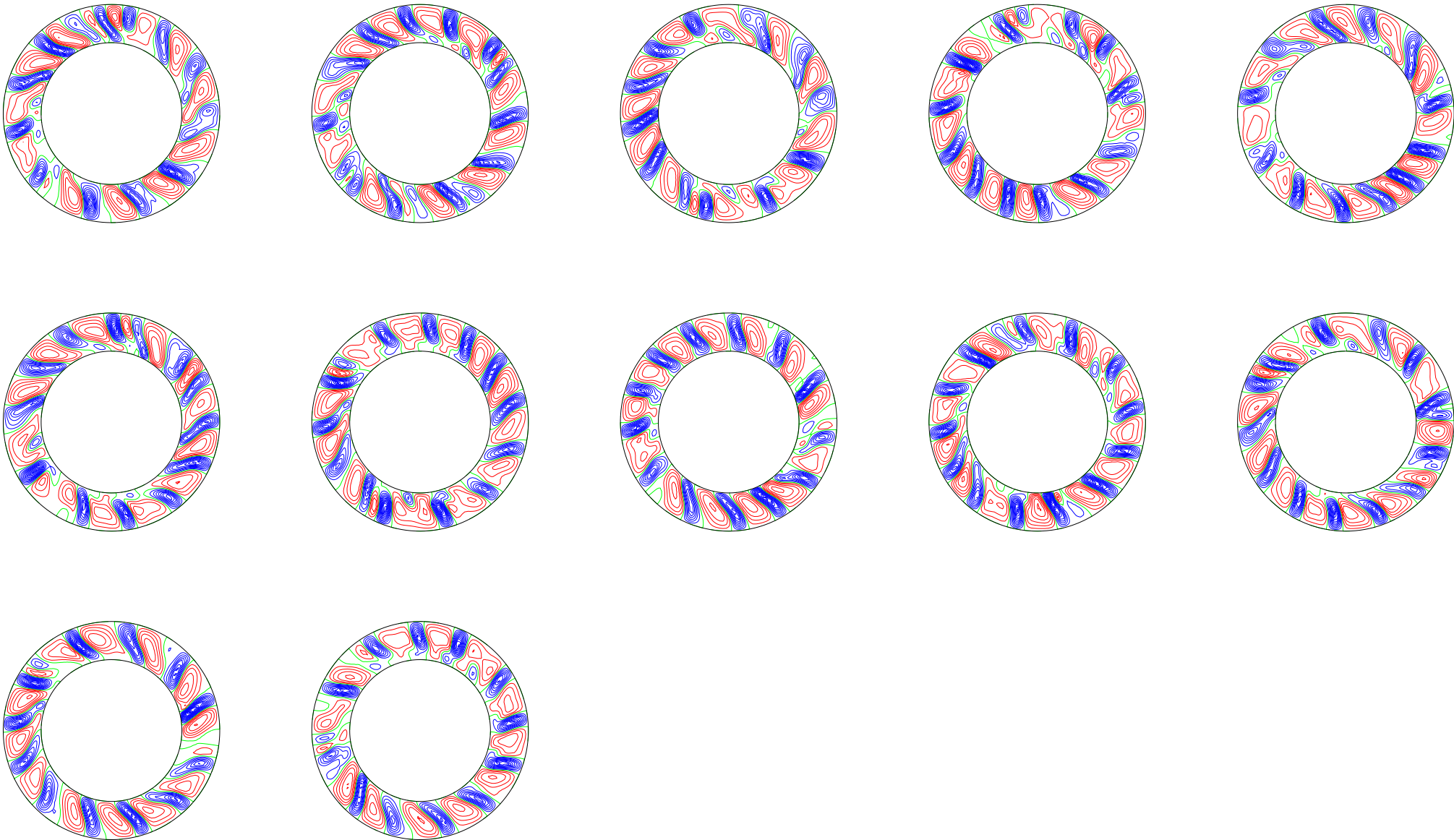
poloidal streamlines, (t[i] dt[i] t[i+1]): 3.150063 ( 0.15 ) 4.800096
