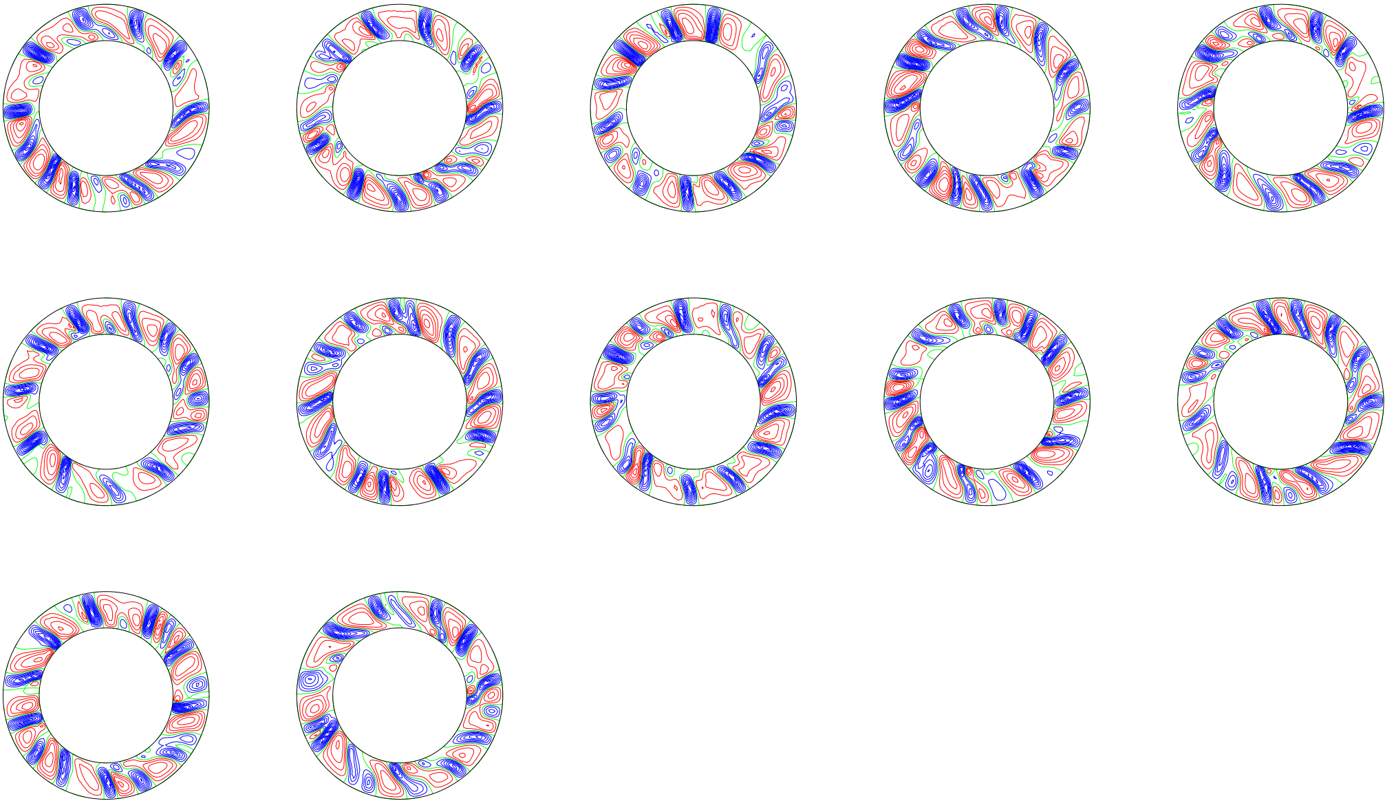
poloidal streamlines, (t[i] dt[i] t[i+1]): 1.200024 ( 0.15 ) 2.850057
