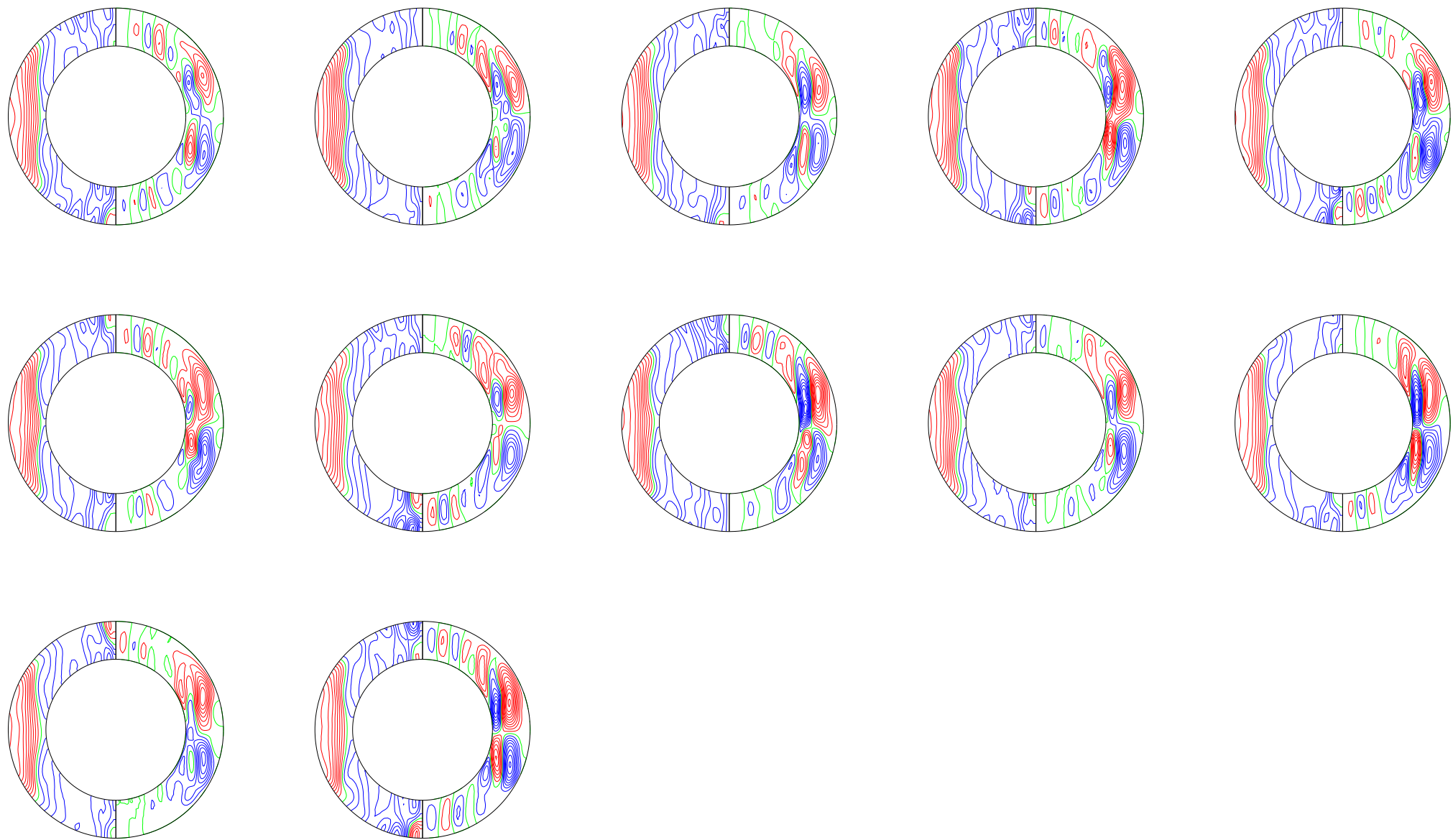
Uphi & merid strlines (merid. cut), (t[i] dt[i] t[i+1]): 2.850057 ( 0.15 ) 4.50009
