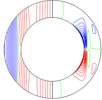
\bar{u}_\phi & merid circulation (mer)
