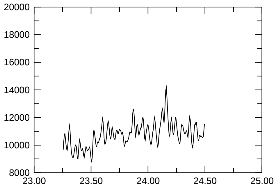
a.e065p1t2r1800000m1p8N3.mv.vc E_{\text{magn}}
