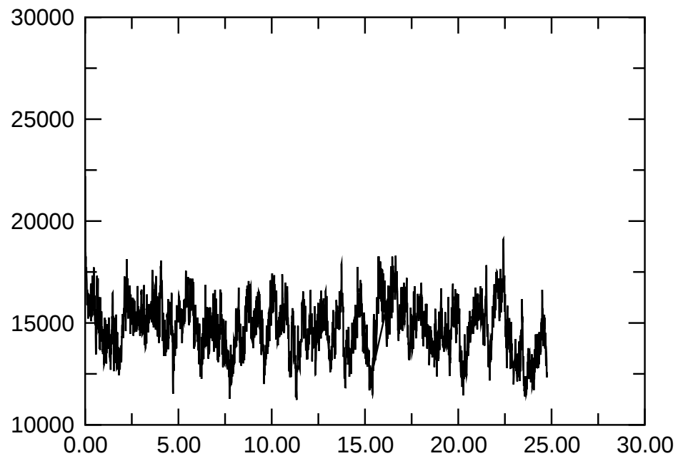
a.e065p1t2r2000000m1p6N3.mv.vc E_{\text{magn}}
