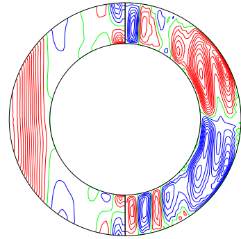
\bar{u}_\varphi & merid circulation (mer) (time-average 0.800008 to 1.00001)
