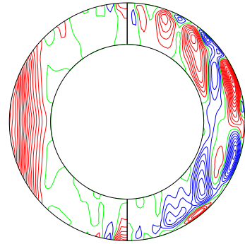
\bar{u}_\varphi & merid circulation (mer) (time-average 22.17315 to 22.27315)
