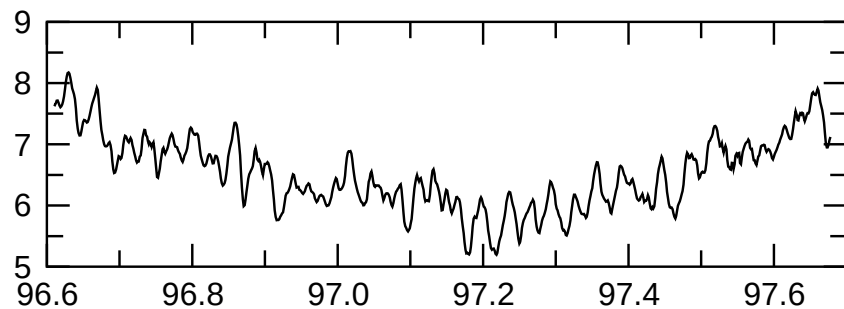
Btor( l=2, m=2 ) magn.
