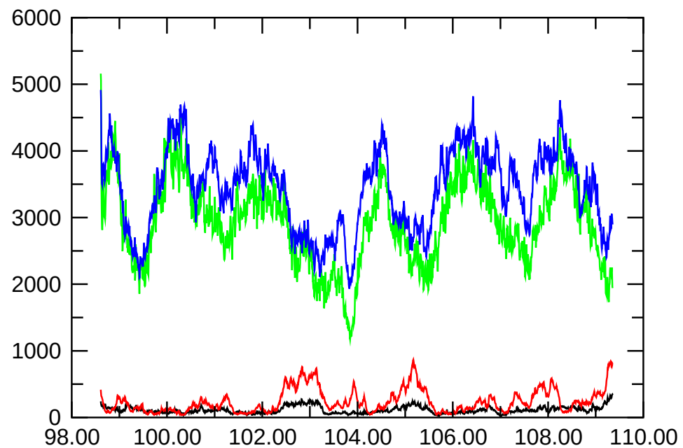
E_{\text{magn,dip.}}
