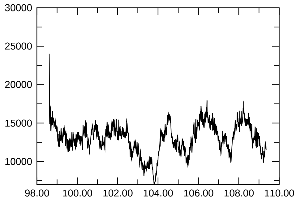
a.mv.e065p1t2r2500000m1p4n1.5N3 E_{\text{magn}}
