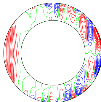
\bar{u}_\varphi & merid circulation (mer) (time-average 21.77315 to 21.97315)
