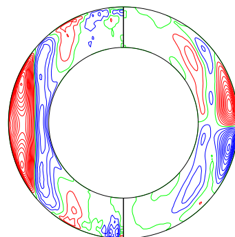
\bar{u}_\varphi & merid circulation (mer) (time-average 14.48815 to 14.52315)
