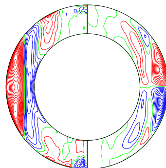
\bar{u}_\phi & merid circulation (mer) (time-average 15.64315 to 15.67815)
