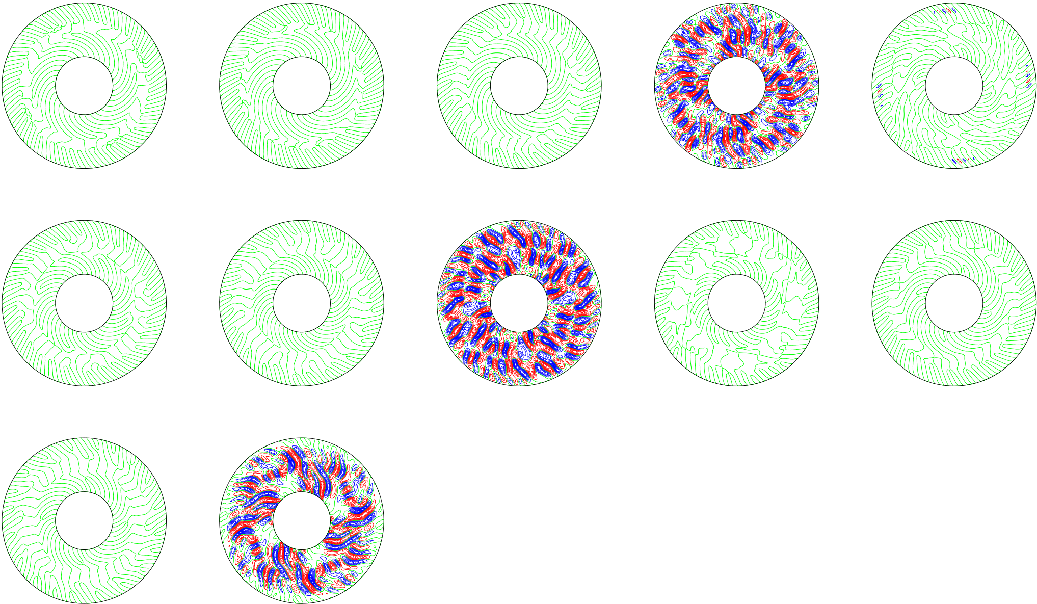
poloidal streamlines, (t[i] dt[i] t[i+1]): 2.640098 ( 0.02 ) 2.860109
