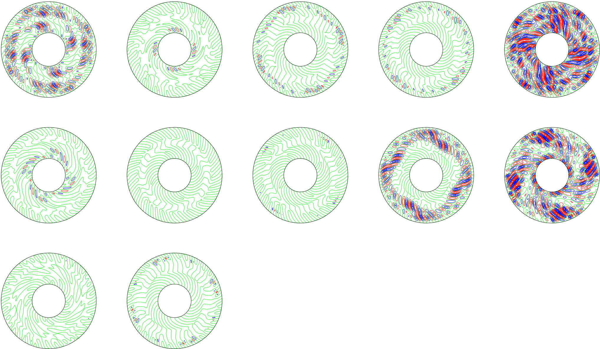
poloidal streamlines, (t[i] dt[i] t[i+1]): 3.360134 ( 0.02 ) 3.580145
