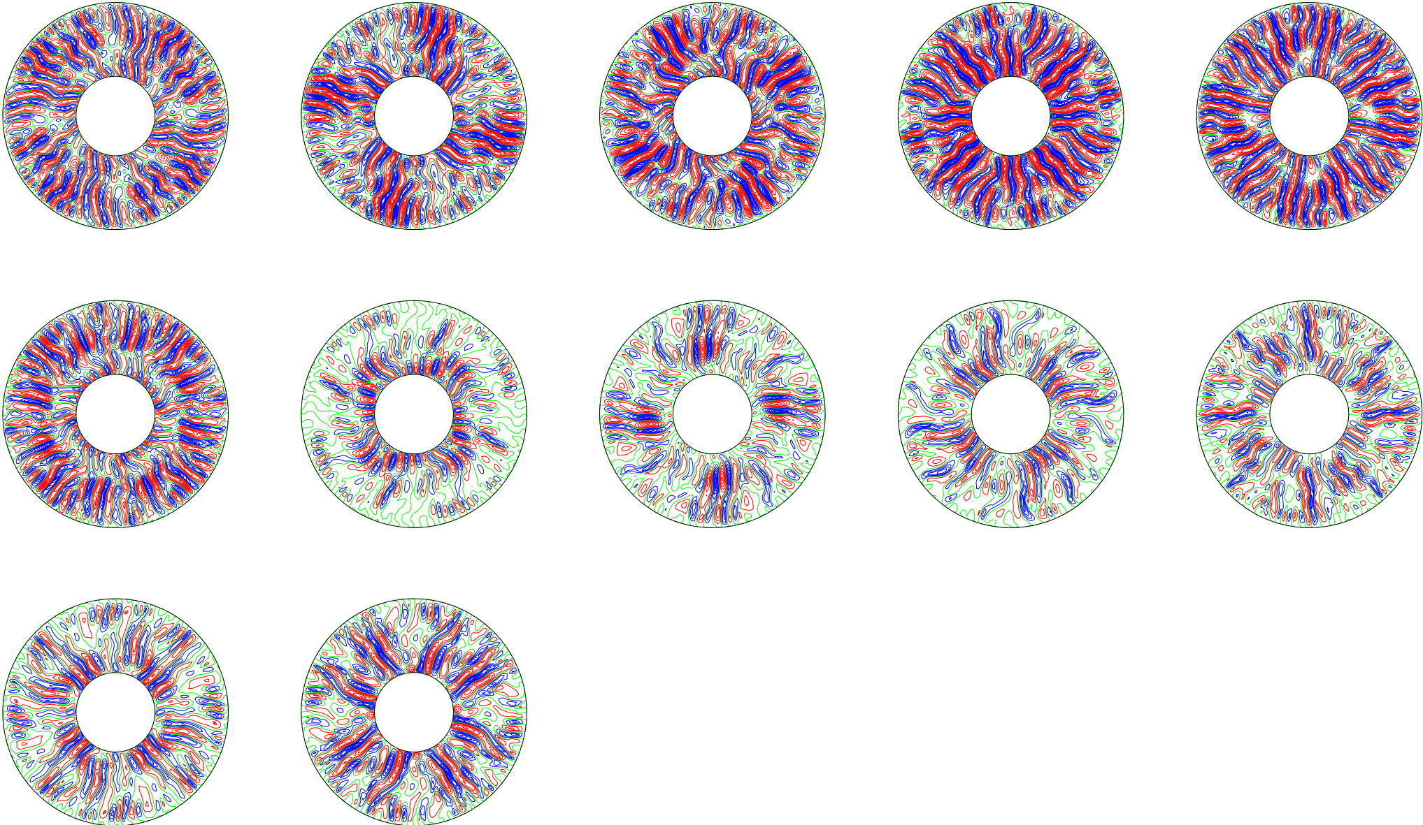
poloidal streamlines, (t[i] dt[i] t[i+1]): 3.920162 ( 0.02 ) 4.140173
