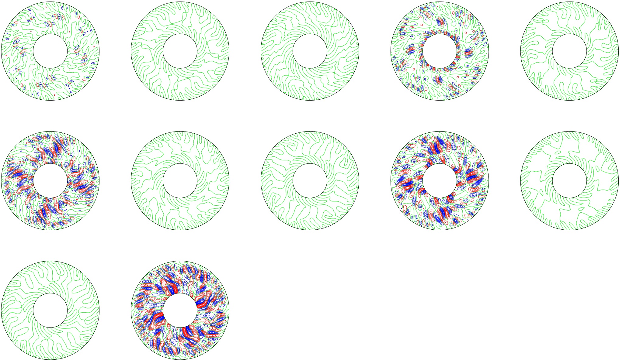
poloidal streamlines, (t[i] dt[i] t[i+1]): 2.88011 ( 0.02 ) 3.100121
