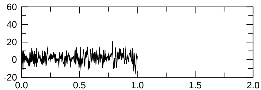
\text{Btor}(l=2, m=2) magn.
