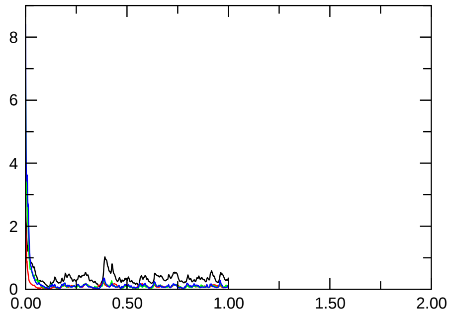
E_{\text{magn,dip.}}
