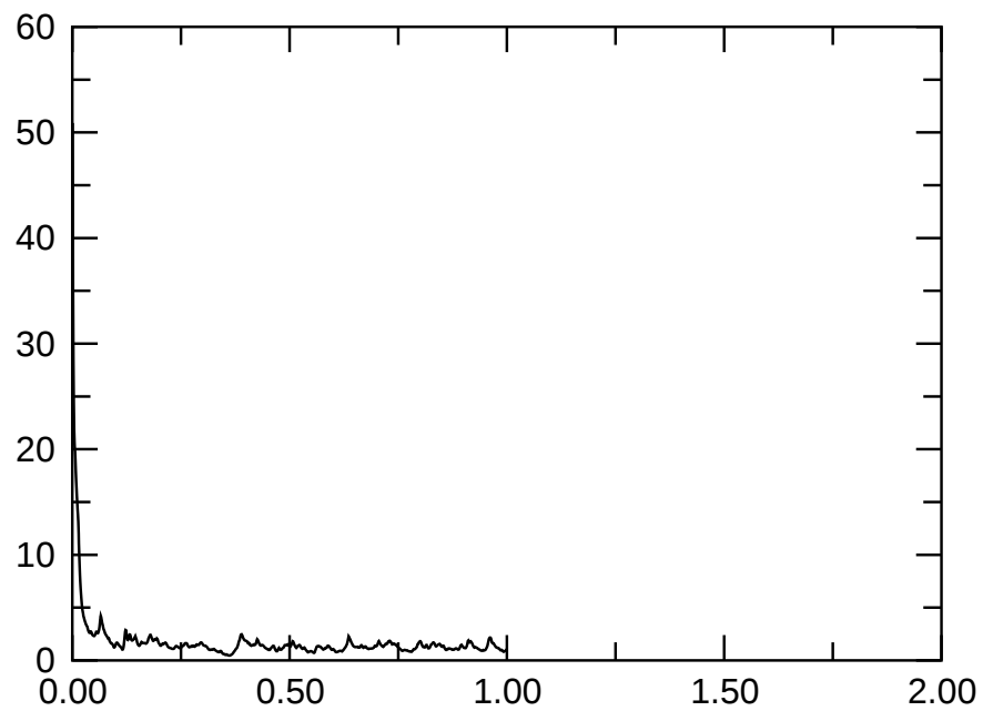
ae035p2t40r15000000m4p2n2Nrho3b E_{\text{magn}}
