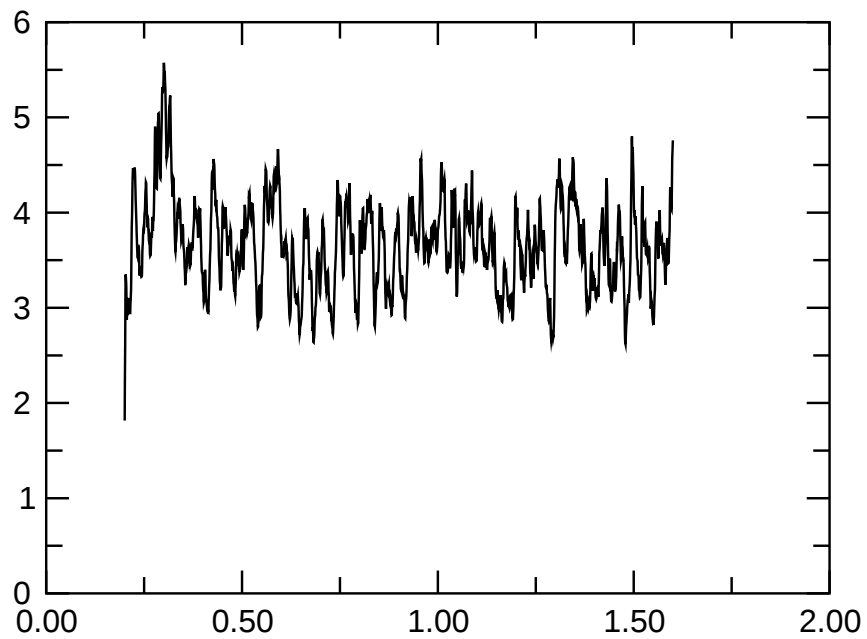
ae035p2t40r20000000m1p2n2Nrho3 E_{\text{magn}}
