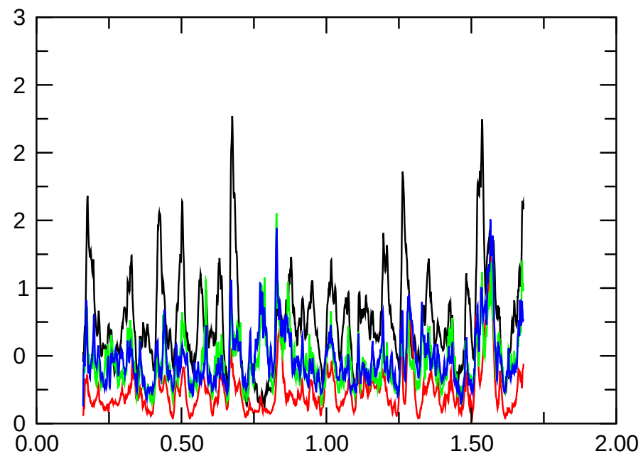
E_{\text{magn,dip.}}
