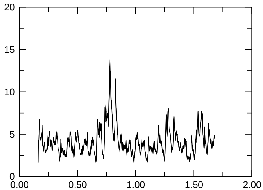
ae035p2t40r20000000m4p2n2Nrho3 E_{\text{magn}}
