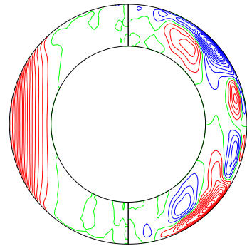
\bar{u}_\varphi & merid circulation (mer) (time-average 14.34815 to 14.38315)
