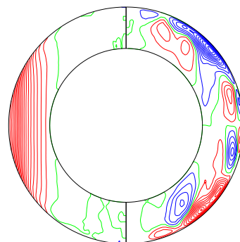
\bar{u}_\varphi & merid circulation (mer) (time-average 14.45315 to 14.48815)
