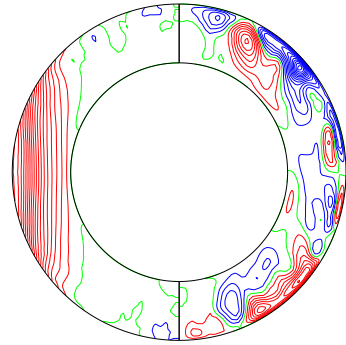
\bar{u}_\varphi & merid circulation (mer) (time-average 14.84815 to 14.86315)
