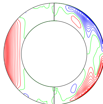
\bar{u}_\varphi & merid circulation (mer) (time-average 15.13815 to 15.18815)
