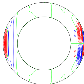
\bar{u}_\phi & merid circulation (mer) (time-average 14.83815 to 14.88815)
