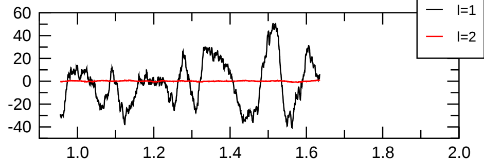
\text{pol}(m=2) magn.
