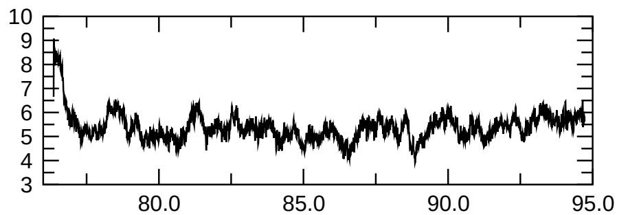
Btor(l=2,m=2) magn.
