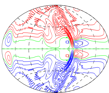
B_r at r = 0.98
