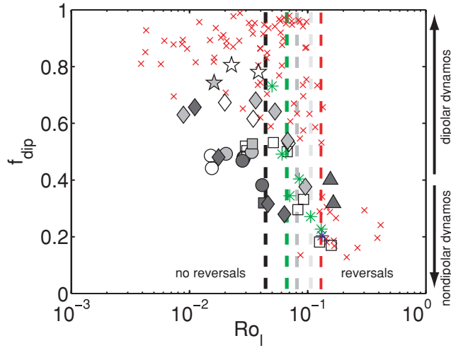
Figure 6. Dipolar fraction f_{\text{dip}} as a function of the local Rossby number Ro_l = Ro/\pi . Symbols as in Fig. 3. The dashed lines delineate the transition point from stable to reversing dynamos: red dashes for the \chi = 0.35 models from Christensen & Aubert (2006), green for \chi = 0.35 and f_i > 1 , light grey for \chi = 0.01\text{--}0.05 and f_i = 0 , medium grey for \chi = 0.01\text{--}0.05 and f_i = 0.5 , black for \chi = 0.01\text{--}0.05 and f_i = 1 . Our data set is filtered to exclude the non-dynamo run.
