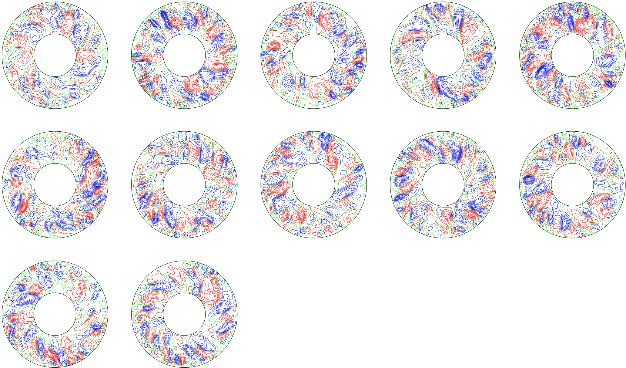
poloidal streamlines, (t[i] dt[i] t[i+1]): 1.350184 ( 0.045 ) 1.845195
