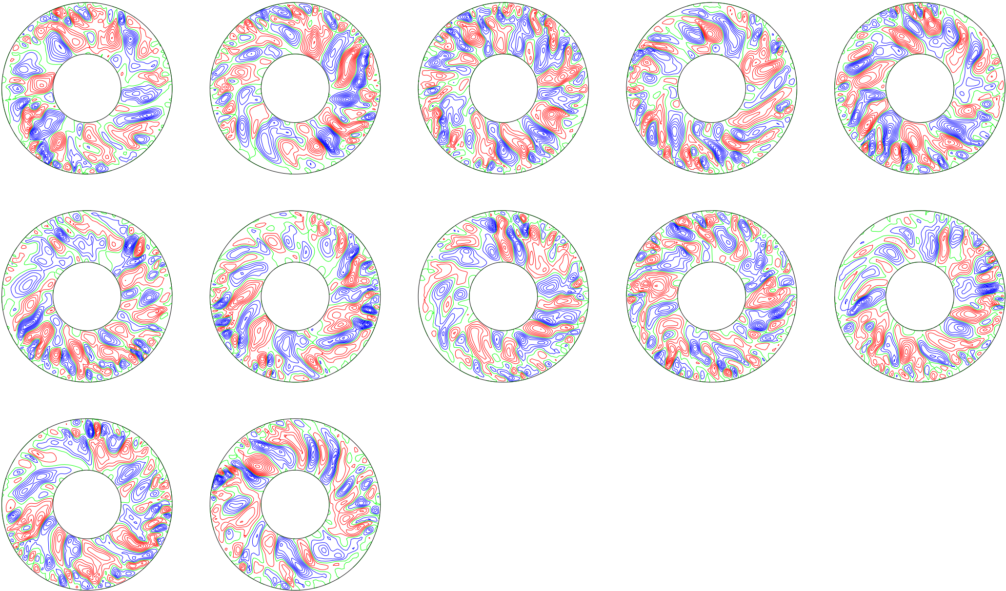
poloidal streamlines, (t[i] dt[i] t[i+1]): 1.890196 ( 0.045 ) 2.385216
